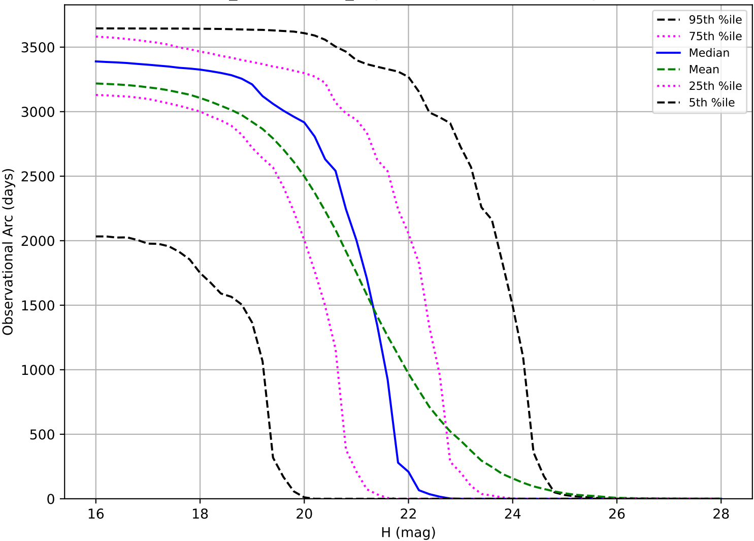
weather_cloudso8v3.4_10yrs: Observational Arc Length PHA
