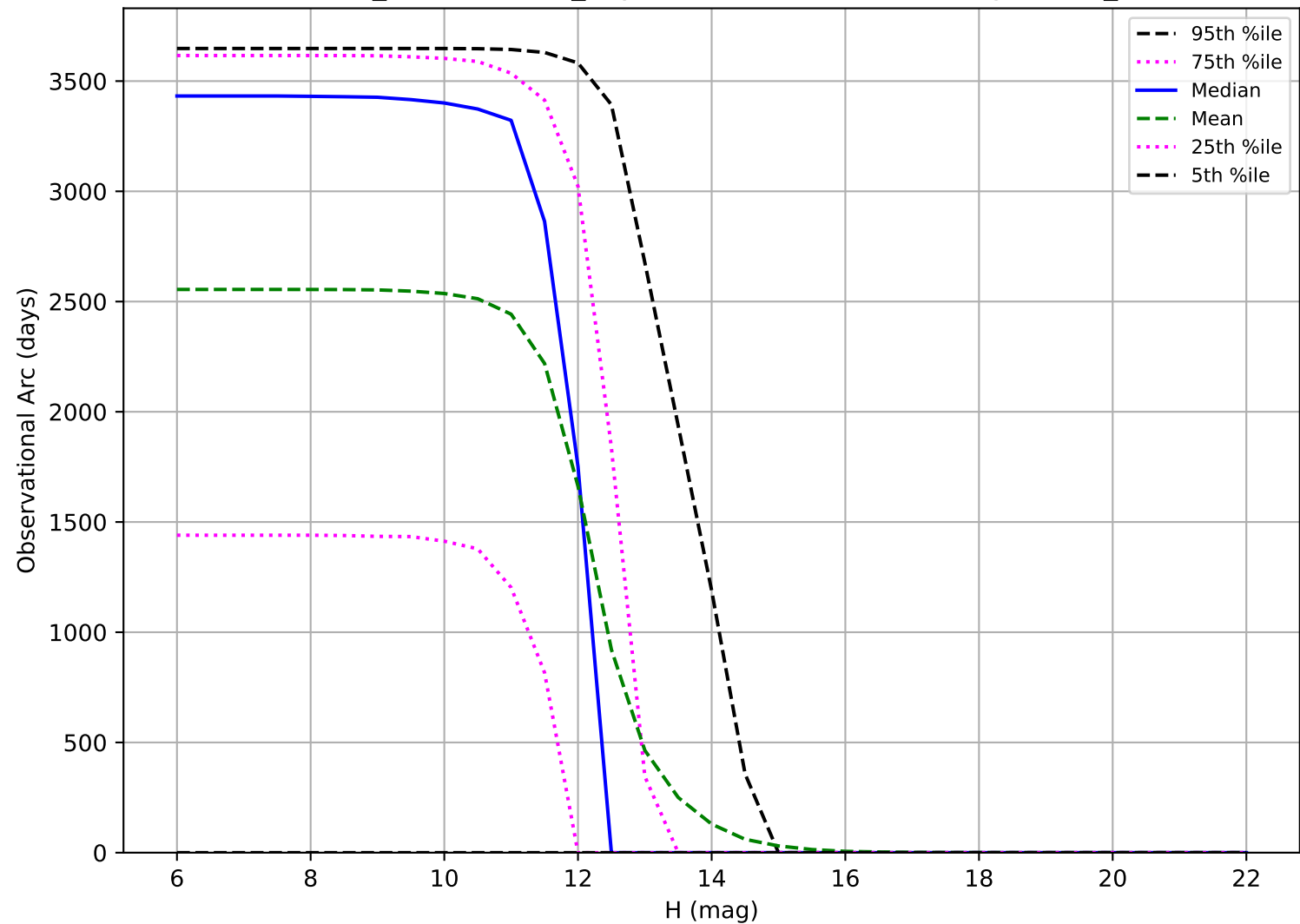
weather_cloudso8v3.4_10yrs: Observational Arc Length OCC_r20
