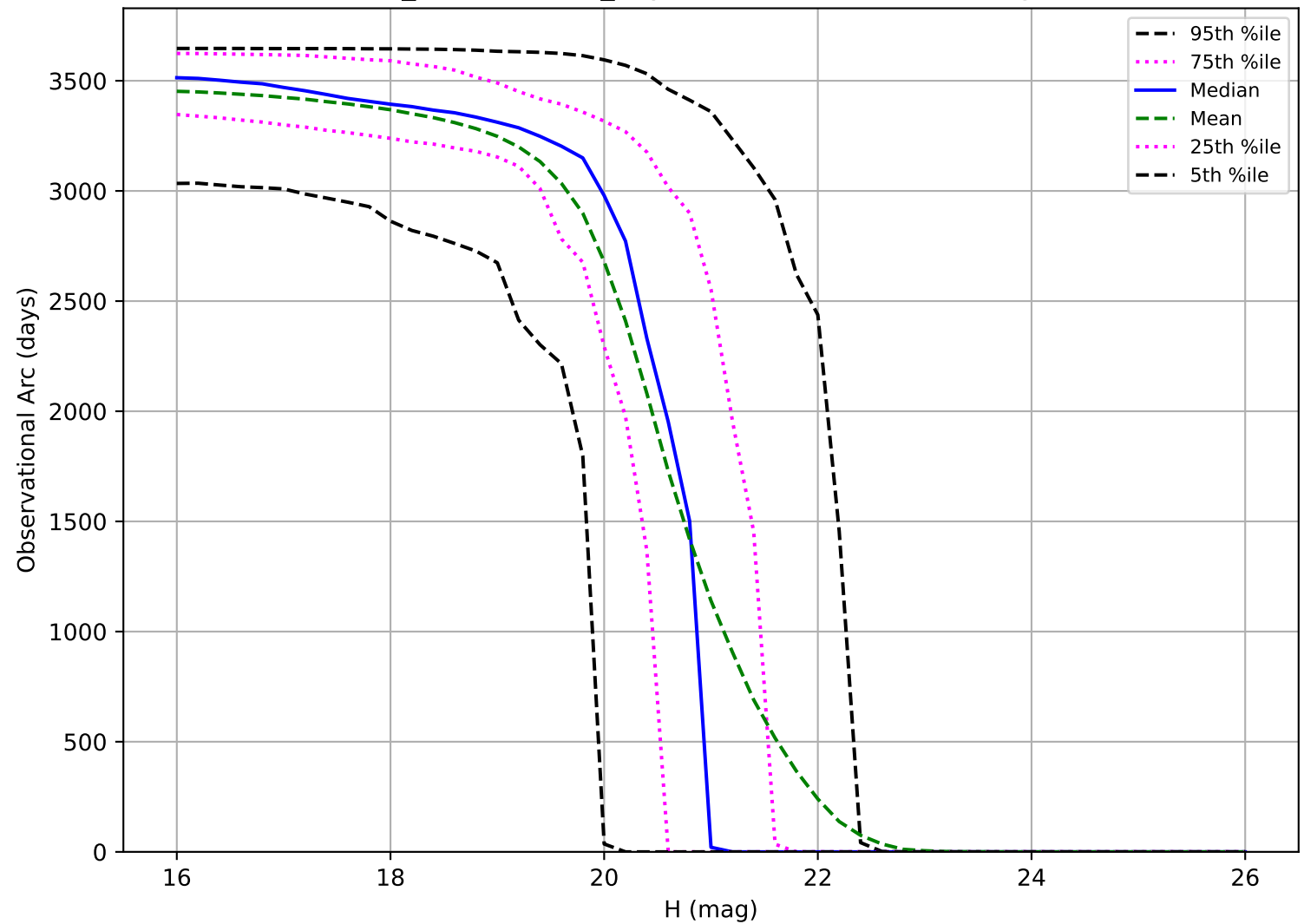
weather_cloudso8v3.4_10yrs: Observational Arc Length MBA
