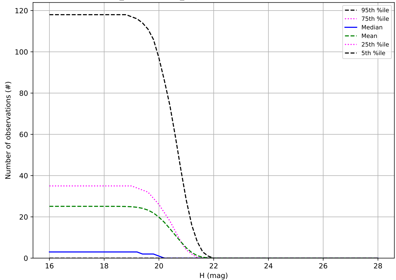
weather_cloudso8v3.4_10yrs: Number of observations Vatira
