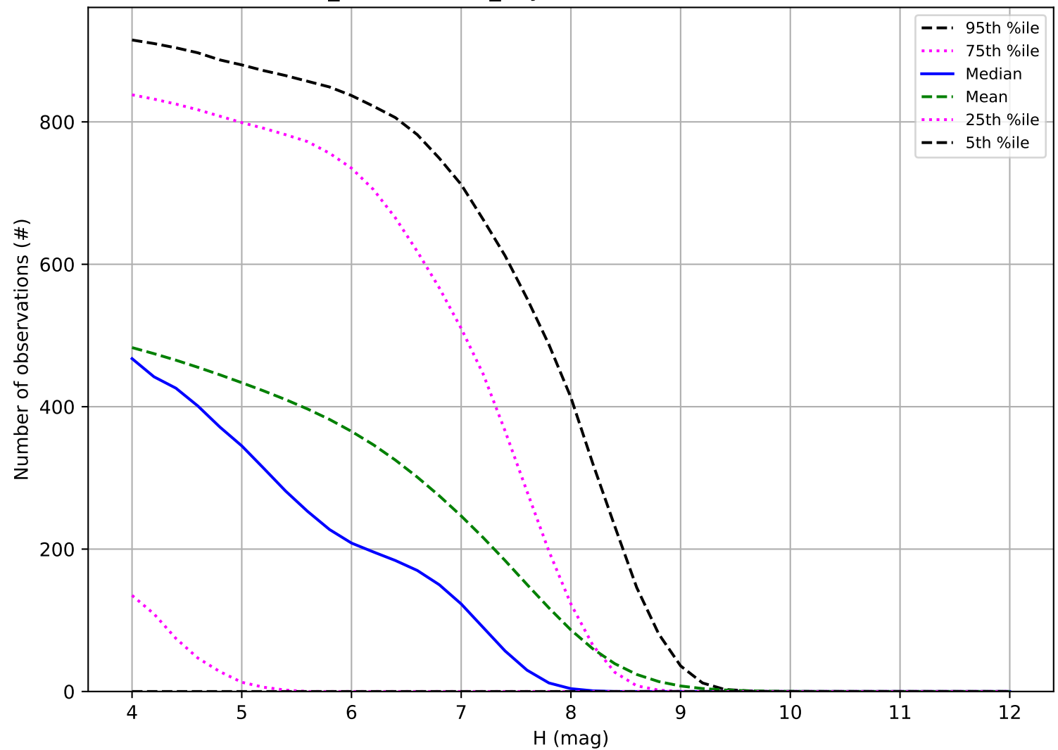
weather_cloudso8v3.4_10yrs: Number of observations TNO
