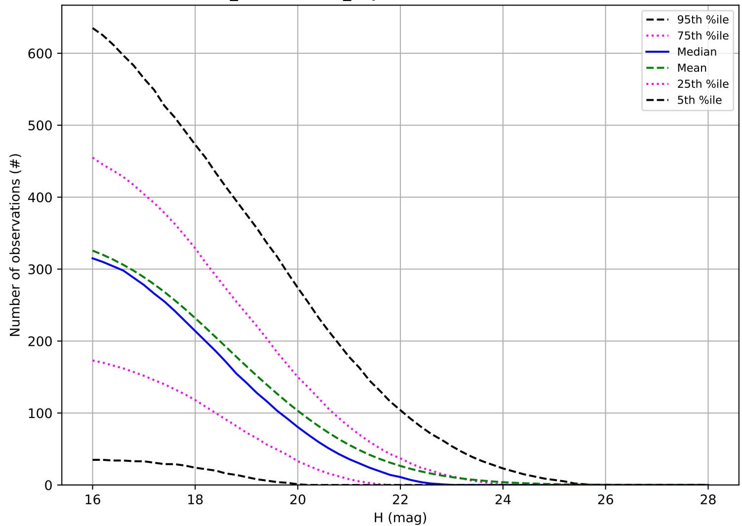
weather_cloudso8v3.4_10yrs: Number of observations NEO
