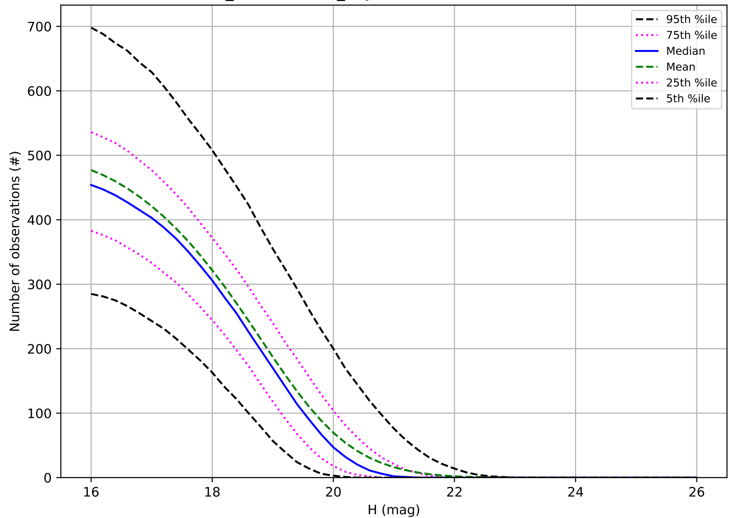
weather_cloudso8v3.4_10yrs: Number of observations MBA
