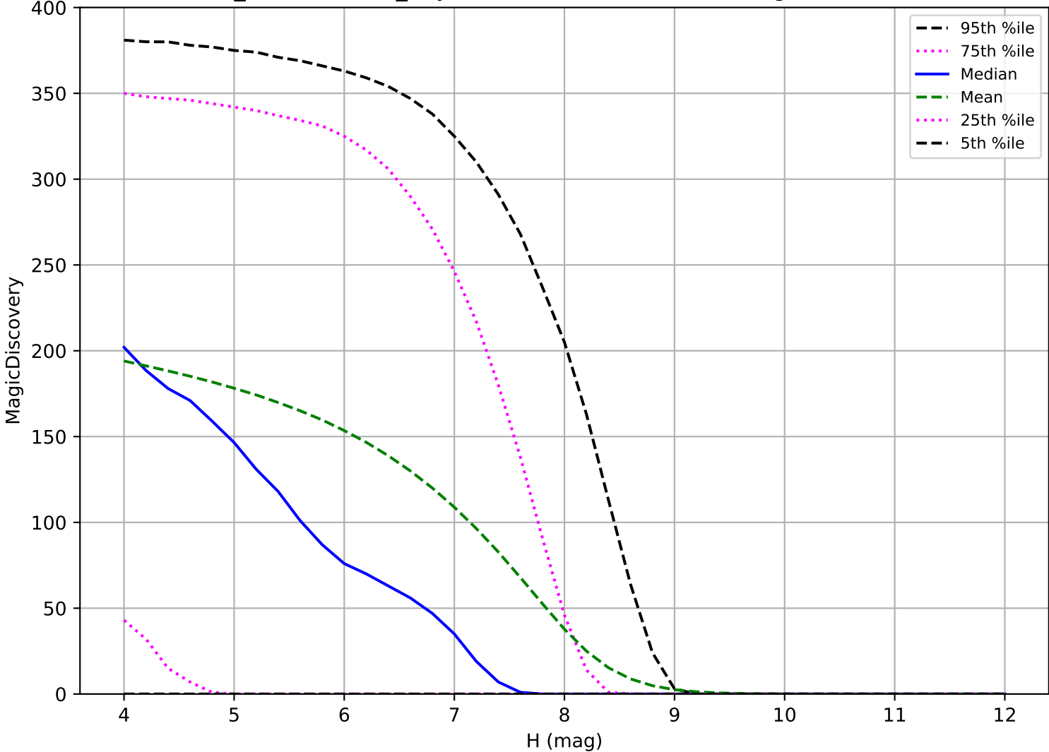
weather_cloudso8v3.4_10yrs: TNO 6 detections in 60 nights detection loss
