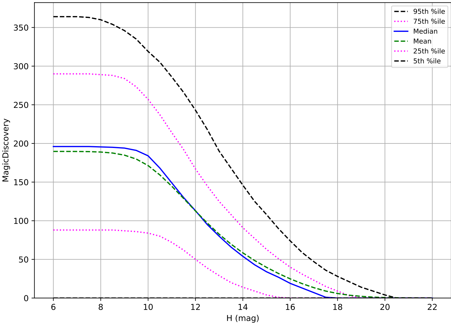
weather_cloudso8v3.4_10yrs: OCC_r5 6 detections in 60 nights detection loss
