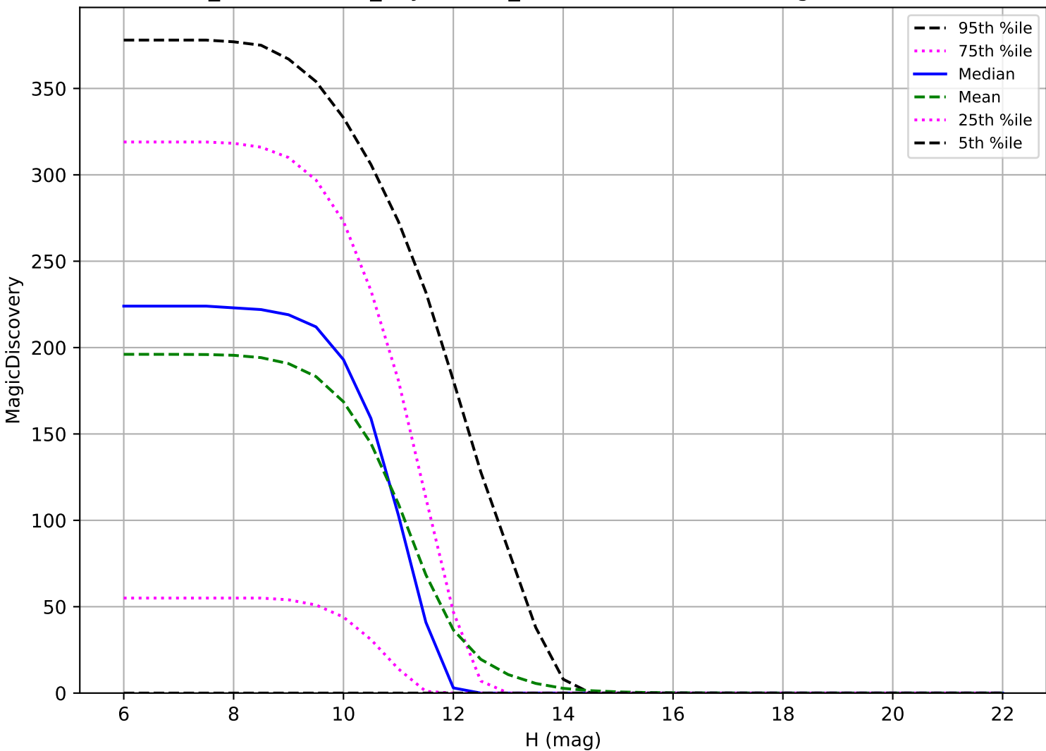
weather_cloudso8v3.4_10yrs: OCC_r20 6 detections in 60 nights detection loss
