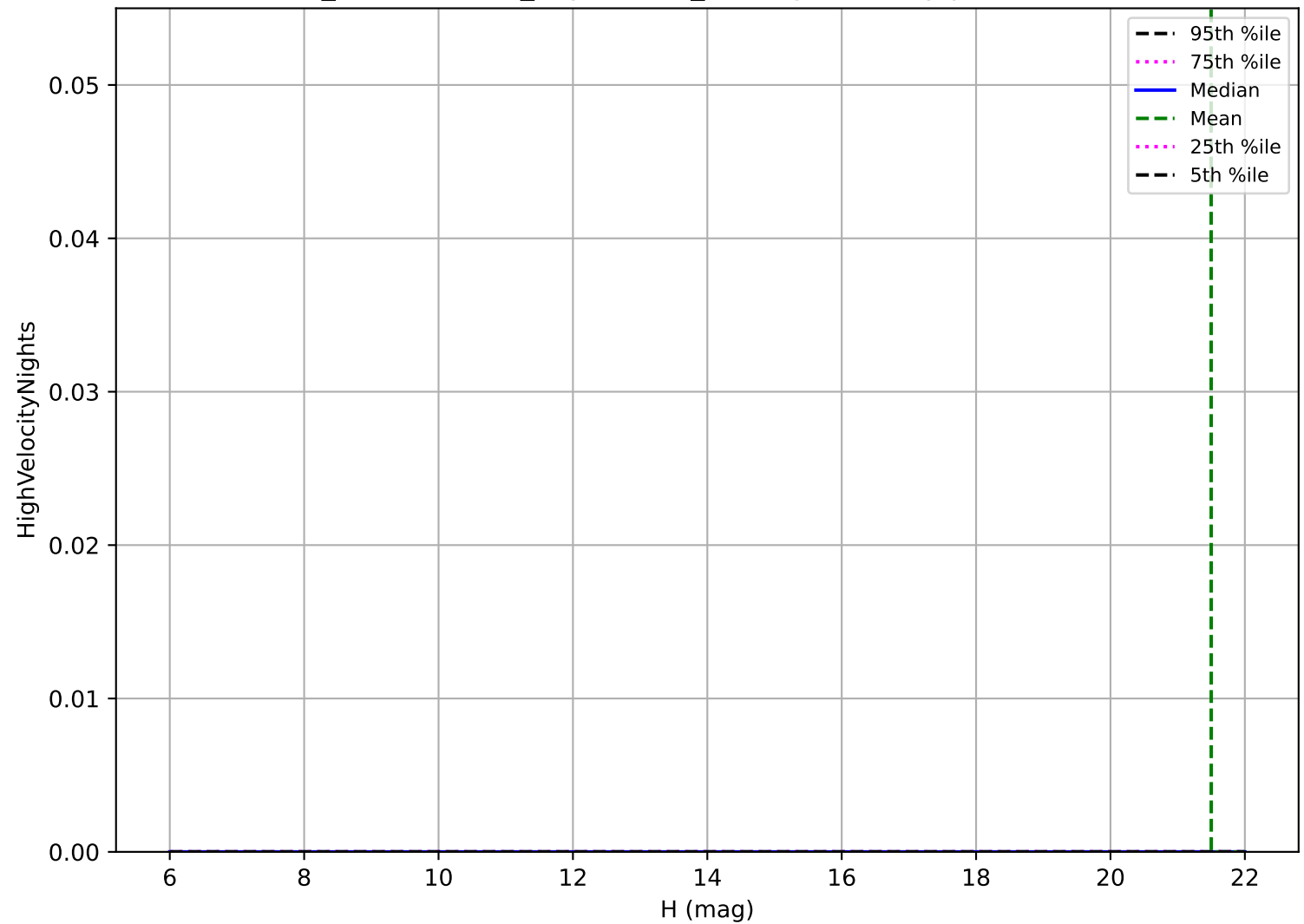
weather_cloudso8v3.4_10yrs: OCC_r20 High velocity pair detection loss
