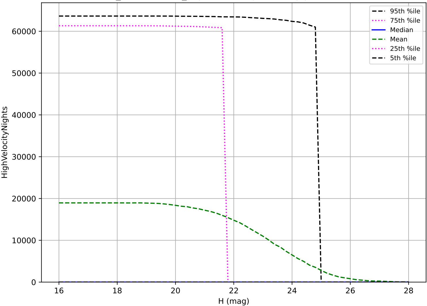
weather_cloudso8v3.4_10yrs: NEO High velocity pair detection loss
