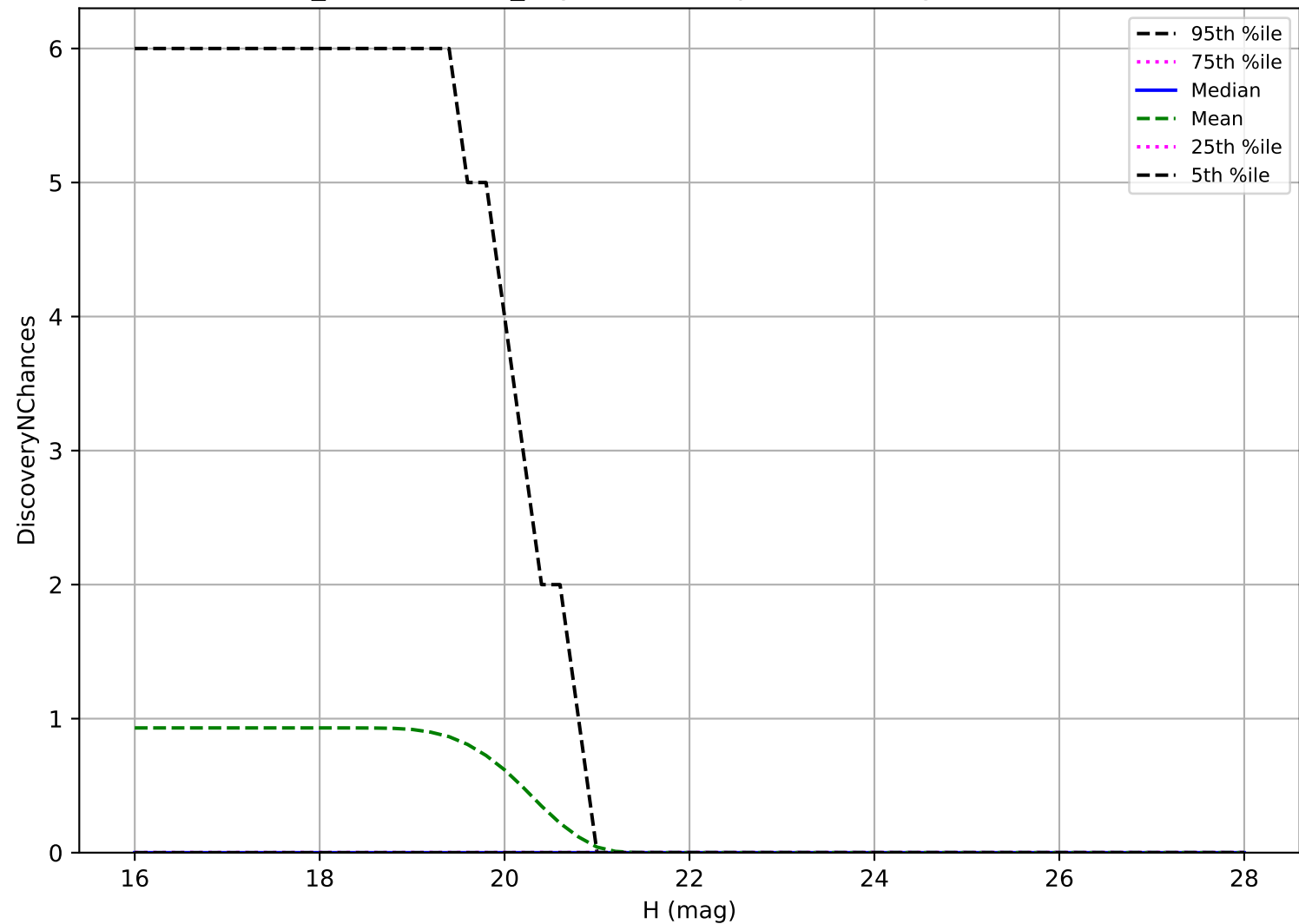
weather_cloudso8v3.4_10yrs: Vatira 3 pairs in 15 nights detection loss
