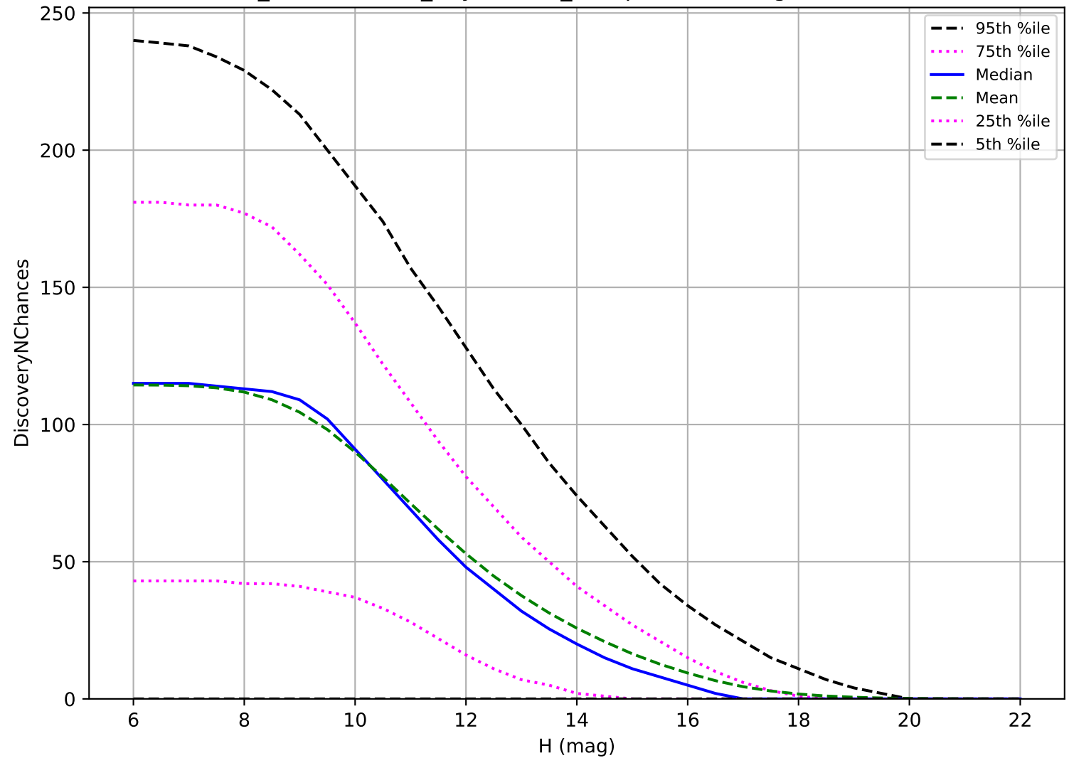
weather_cloudso8v3.4_10yrs: OCC_r5 3 pairs in 15 nights detection loss
