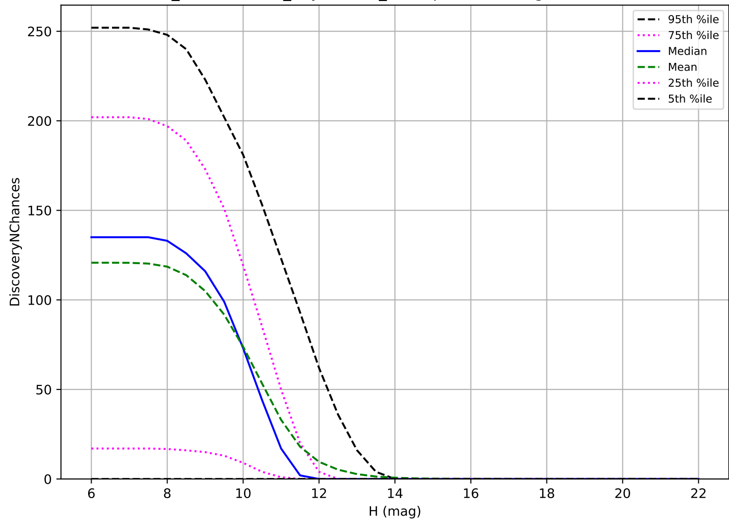
weather_cloudso8v3.4_10yrs: OCC_r20 3 pairs in 15 nights detection loss
