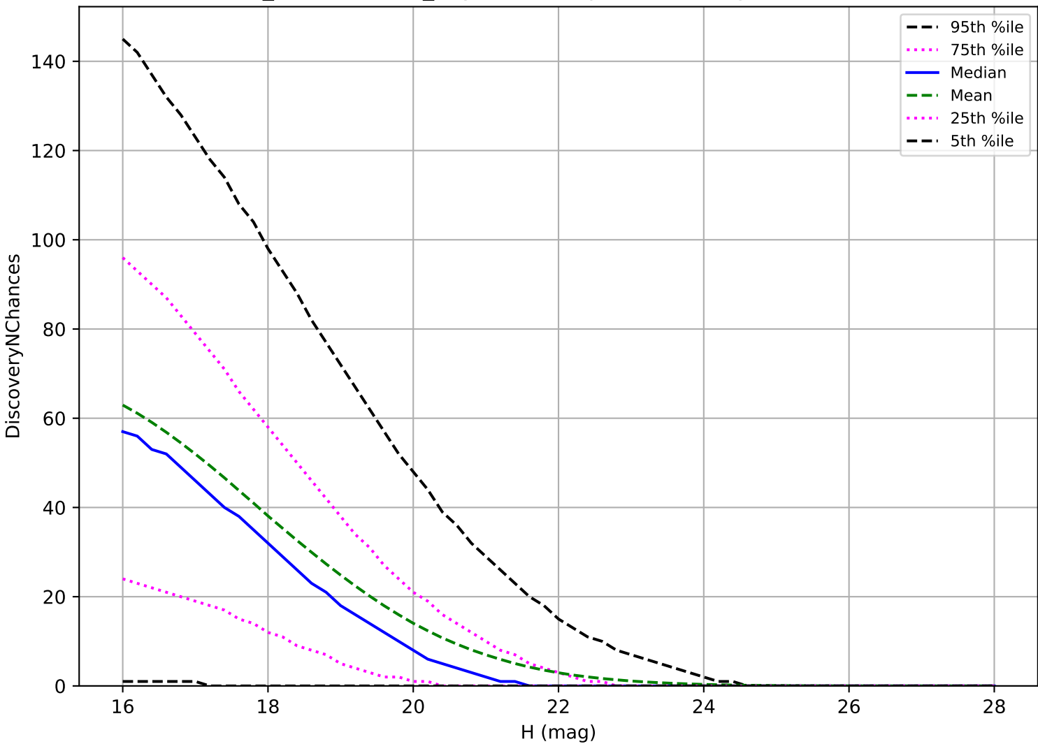
weather_cloudso8v3.4_10yrs: NEO 3 pairs in 15 nights detection loss
