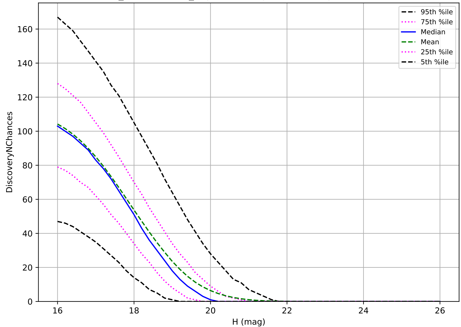
weather_cloudso8v3.4_10yrs: MBA 3 pairs in 15 nights detection loss
