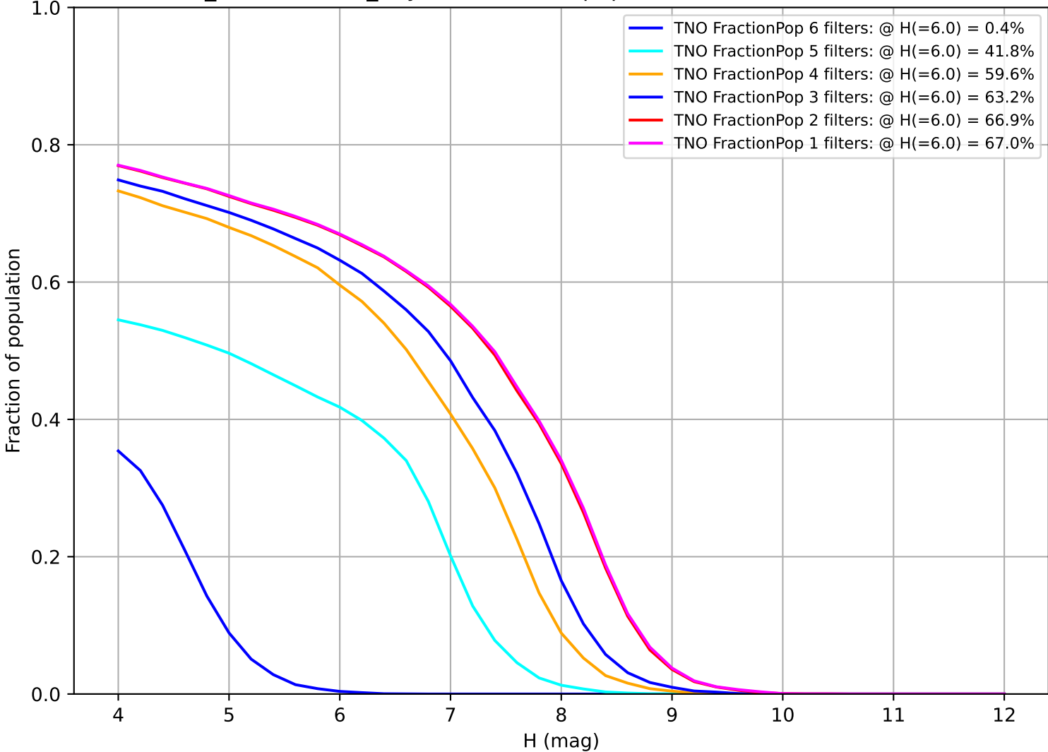
weather_cloudso8v3.4_10yrs: Fraction of population with colors in X filters TNO
