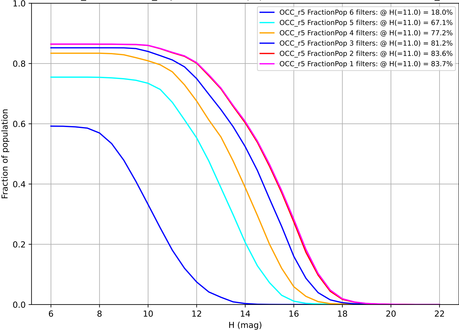
weather_cloudso8v3.4_10yrs: Fraction of population with colors in X filters OCC_r5
