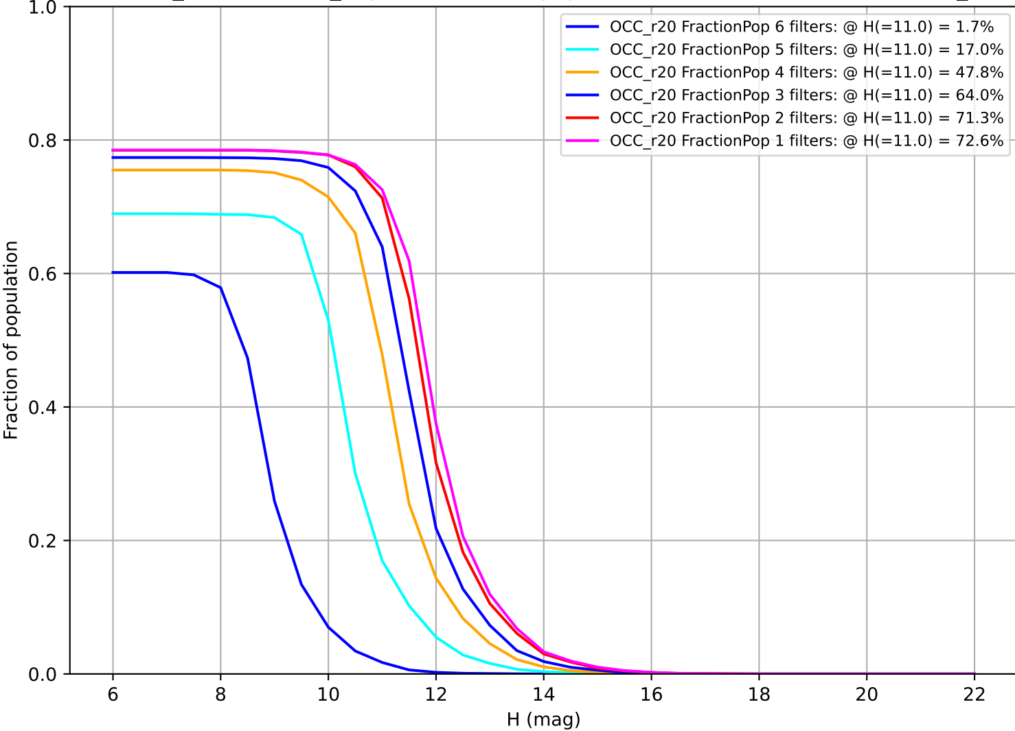
weather_cloudso8v3.4_10yrs: Fraction of population with colors in X filters OCC_r20
