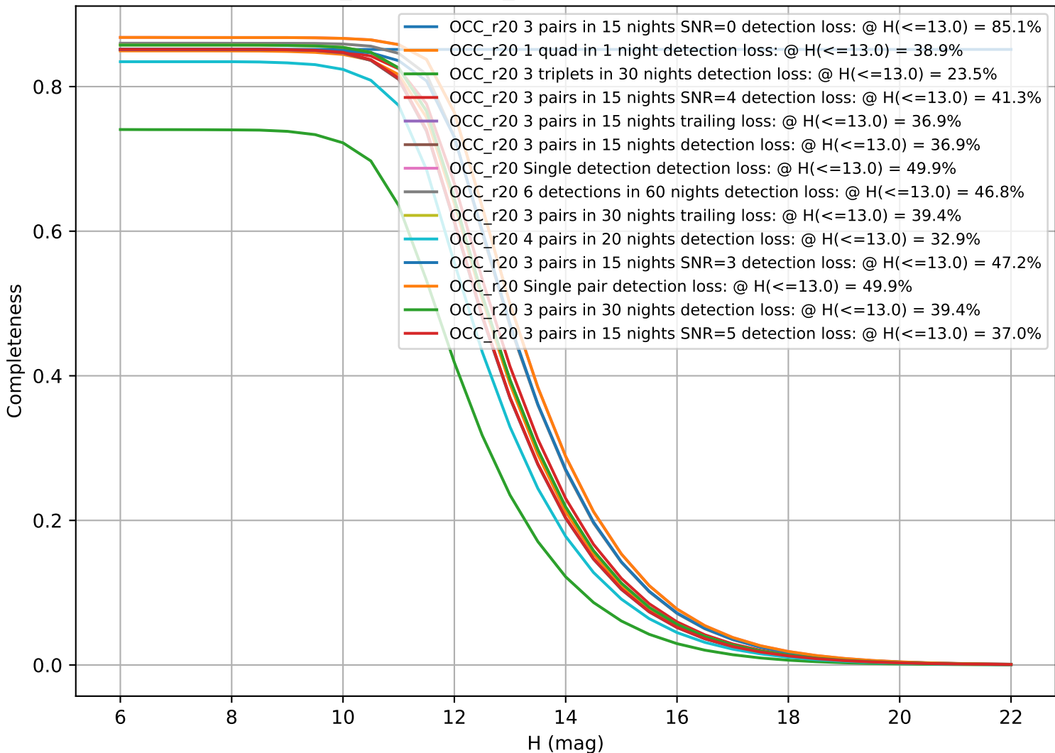
weather_cloudso8v3.4_10yrs: CumulativeCompleteness
