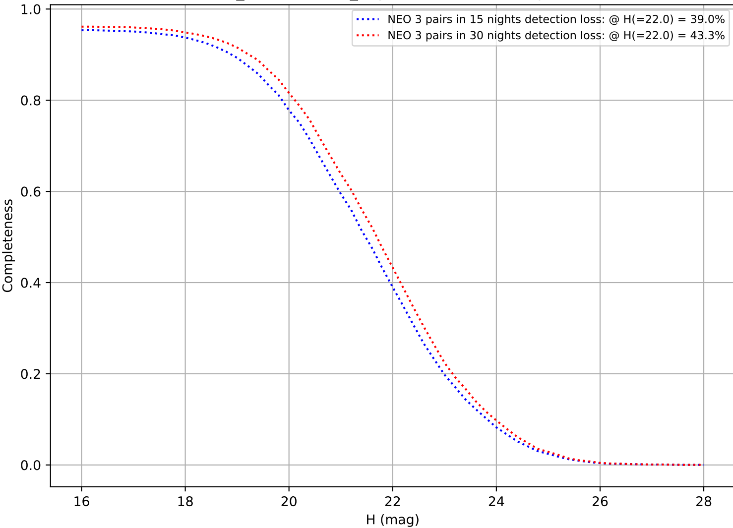
weather_cloudso8v3.4_10yrs: DifferentialCompleteness
