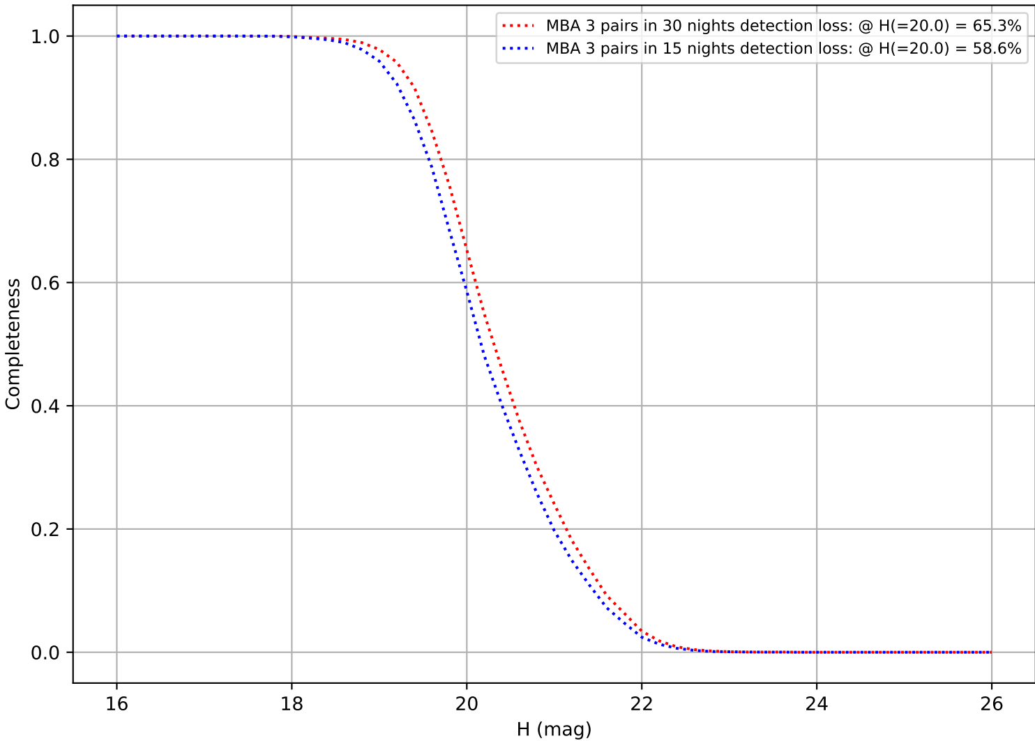
weather_cloudso8v3.4_10yrs: DifferentialCompleteness
