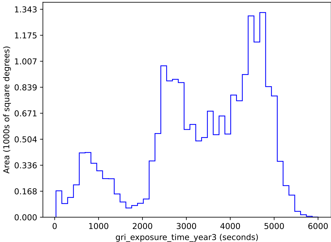
weather_cloudso8v3.4_10yrs gri band non-DD: gri_exposure_time_year3
