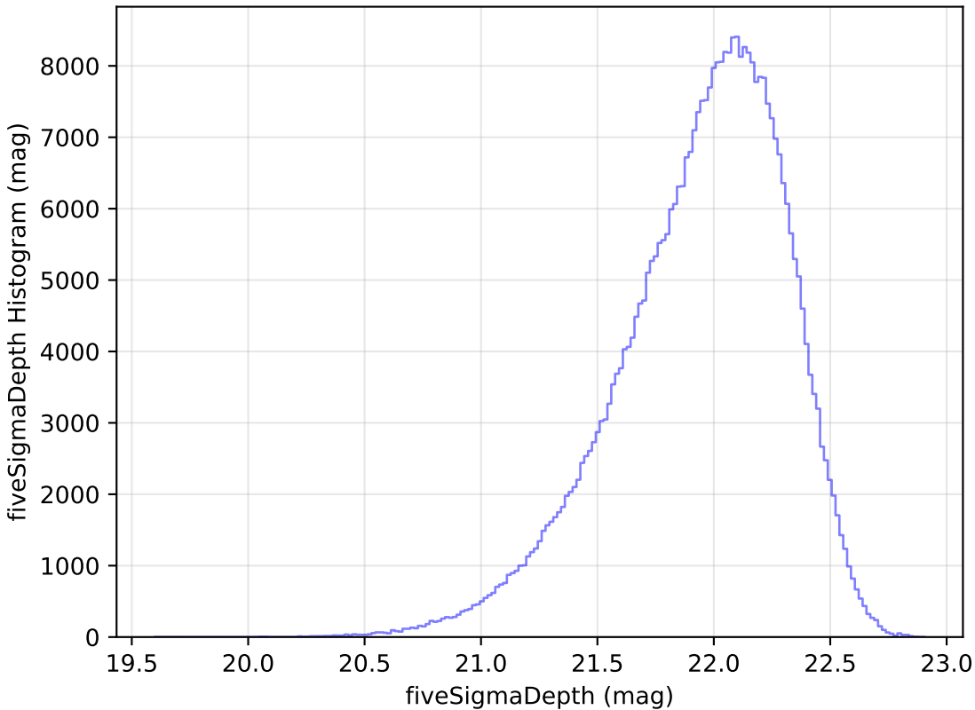
weather_cloudso8v3.4_10yrs y: fiveSigmaDepth Histogram
