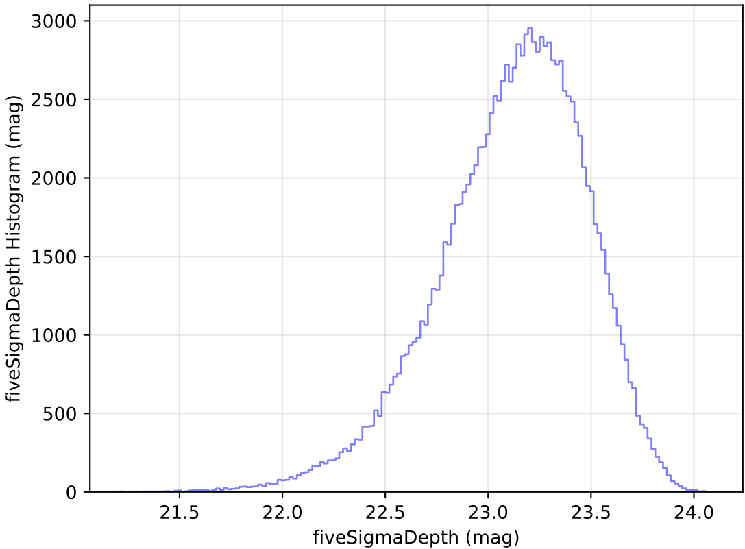
weather_cloudso8v3.4_10yrs u: fiveSigmaDepth Histogram
