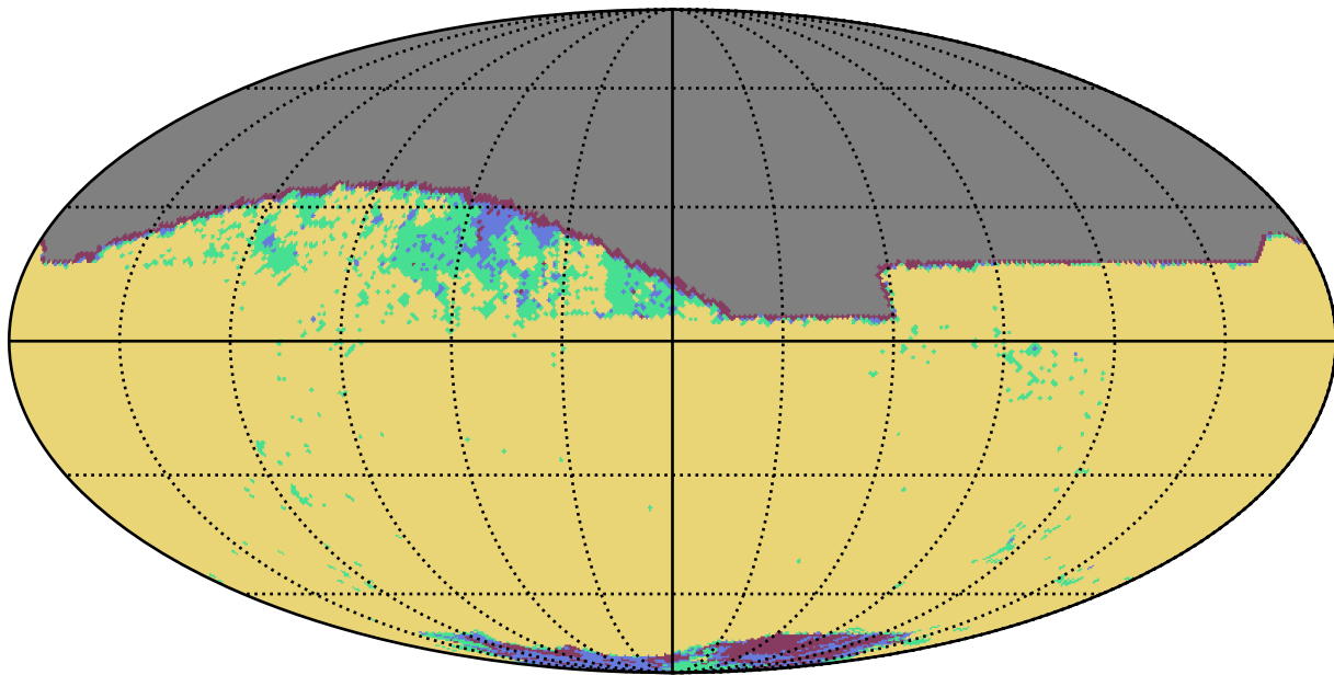
weather_cloudso8v3.4_10yrs z band: YearCoverage night
