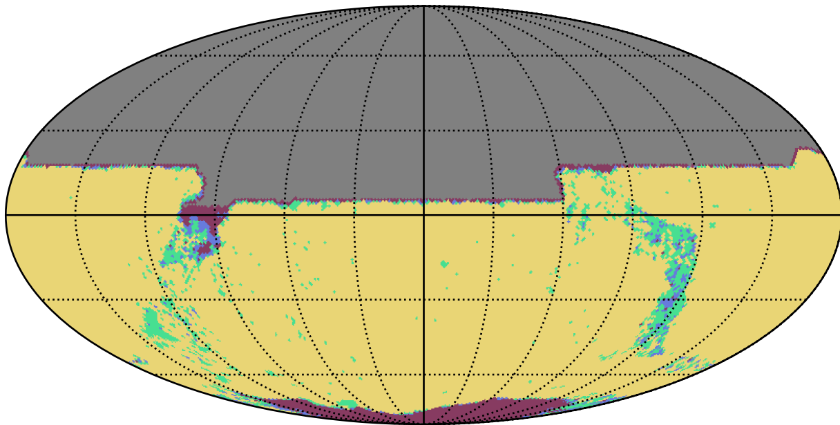
weather_cloudso8v3.4_10yrs y band: YearCoverage night
