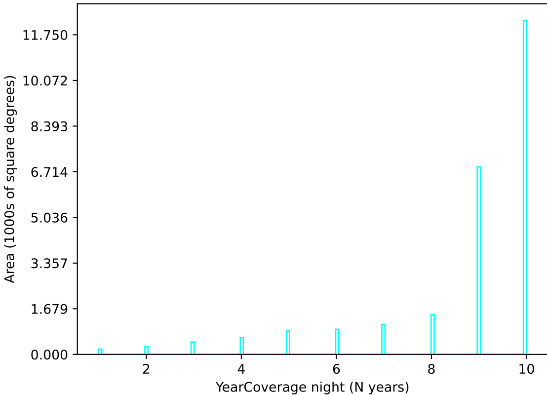
weather_cloudso8v3.4_10yrs u band: YearCoverage night
