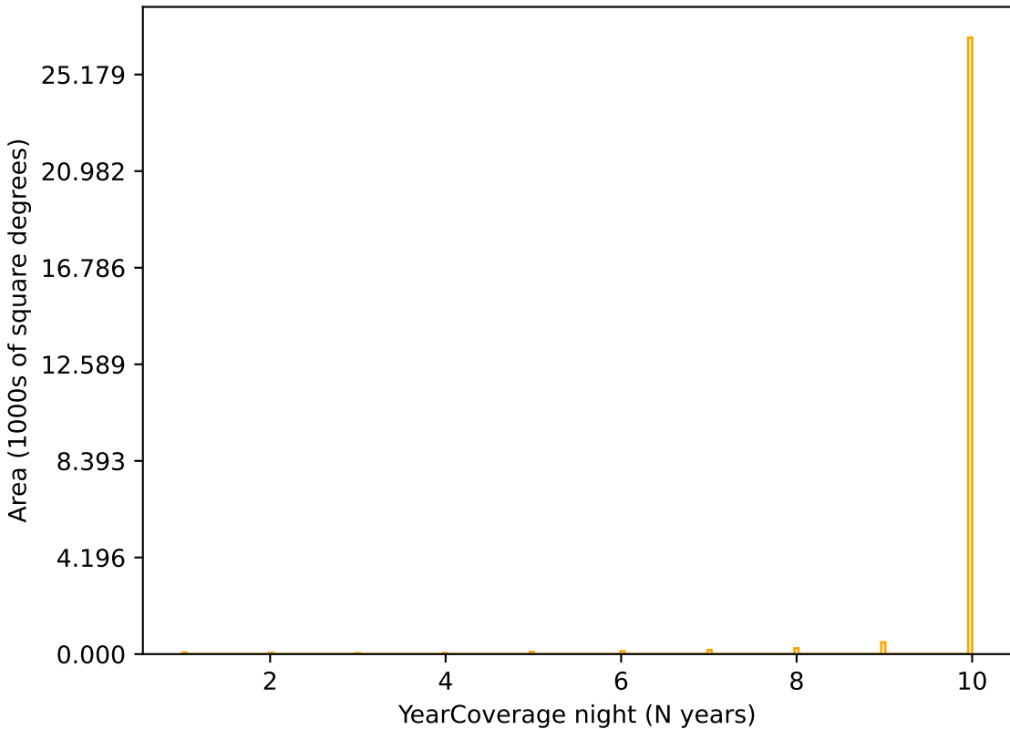
weather_cloudso8v3.4_10yrs r band: YearCoverage night
