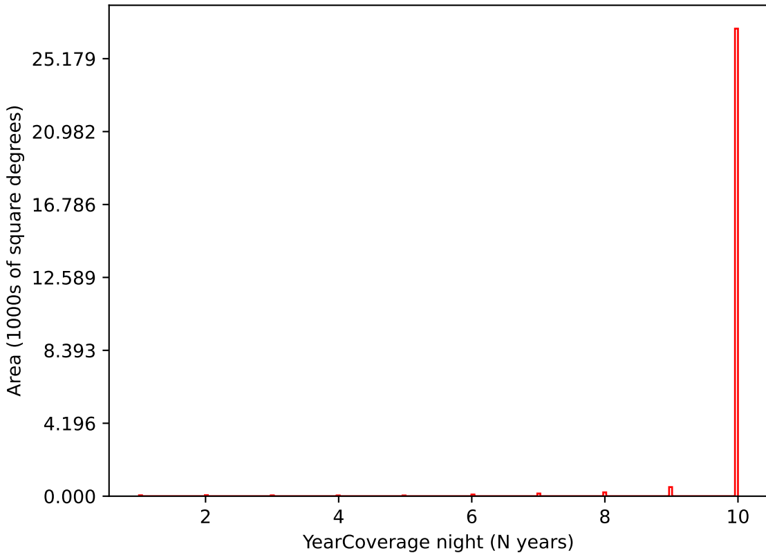
weather_cloudso8v3.4_10yrs i band: YearCoverage night
