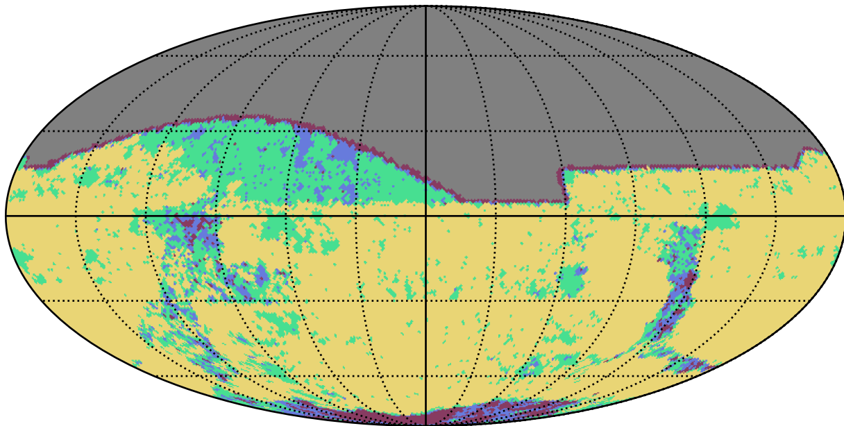
weather_cloudso8v3.4_10yrs g band: YearCoverage night
