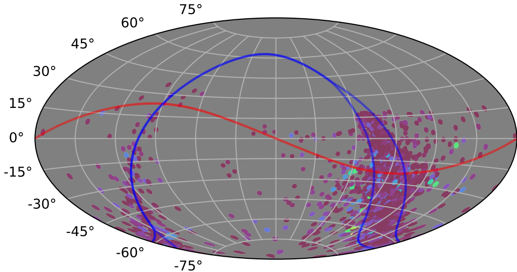
weather_cloudso8v3.4_10yrs : XRBPopMetric_number_of_detections
