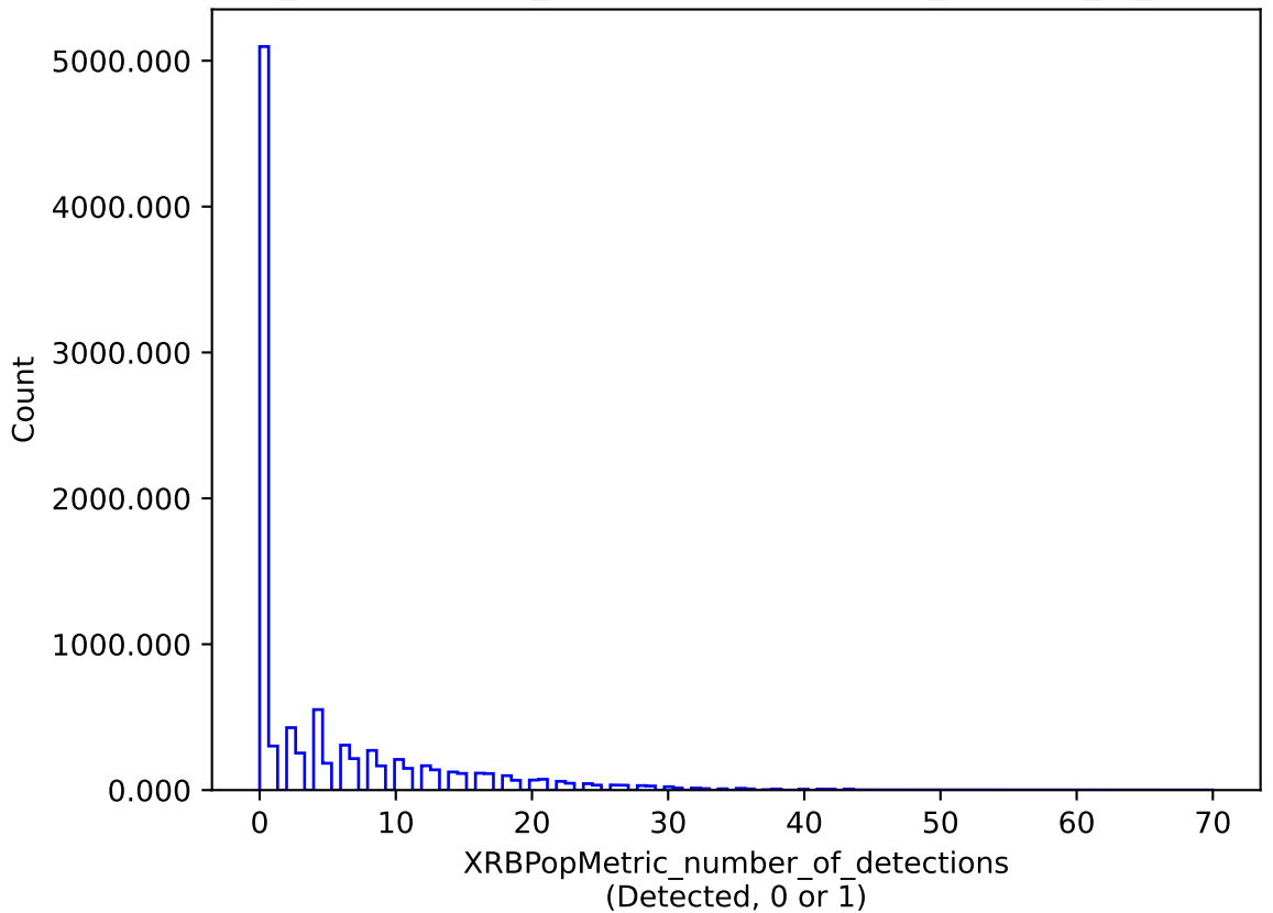
weather_cloudso8v3.4_10yrs : XRBPoMetric_number_of_detections
