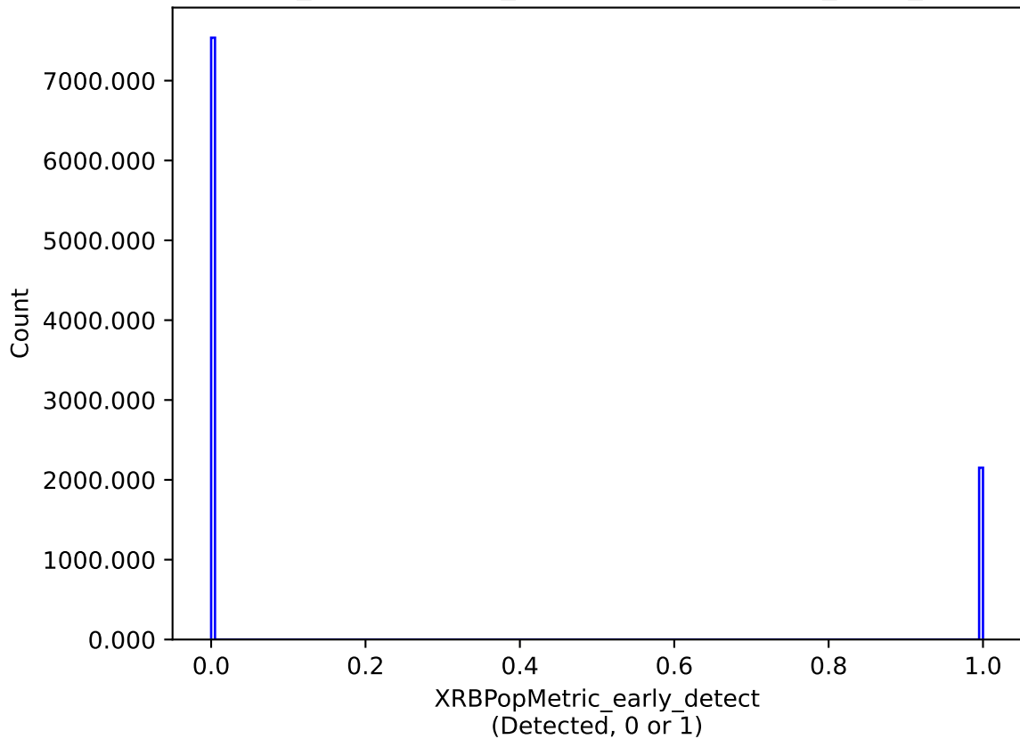
weather_cloudso8v3.4_10yrs : XRBPoMetric_early_detect
