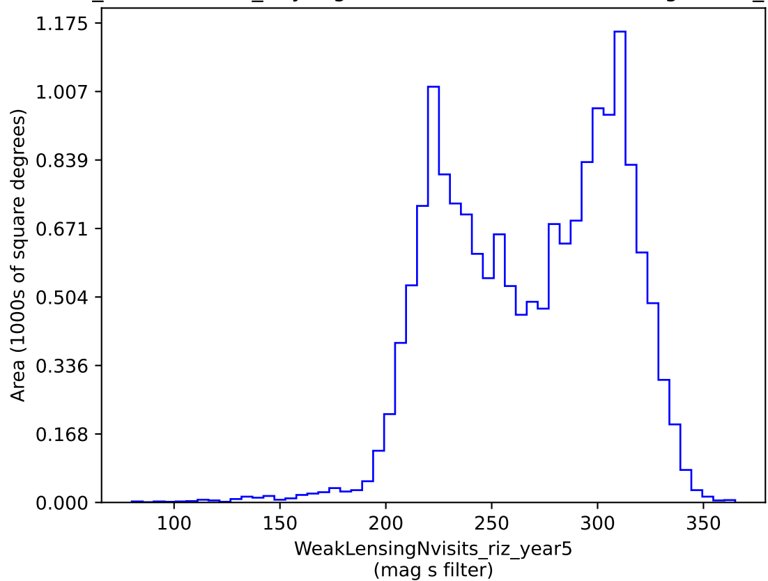
weather_cloudso8v3.4_10yrs gri band non-DD: WeakLensingNvisits_riz_year5
