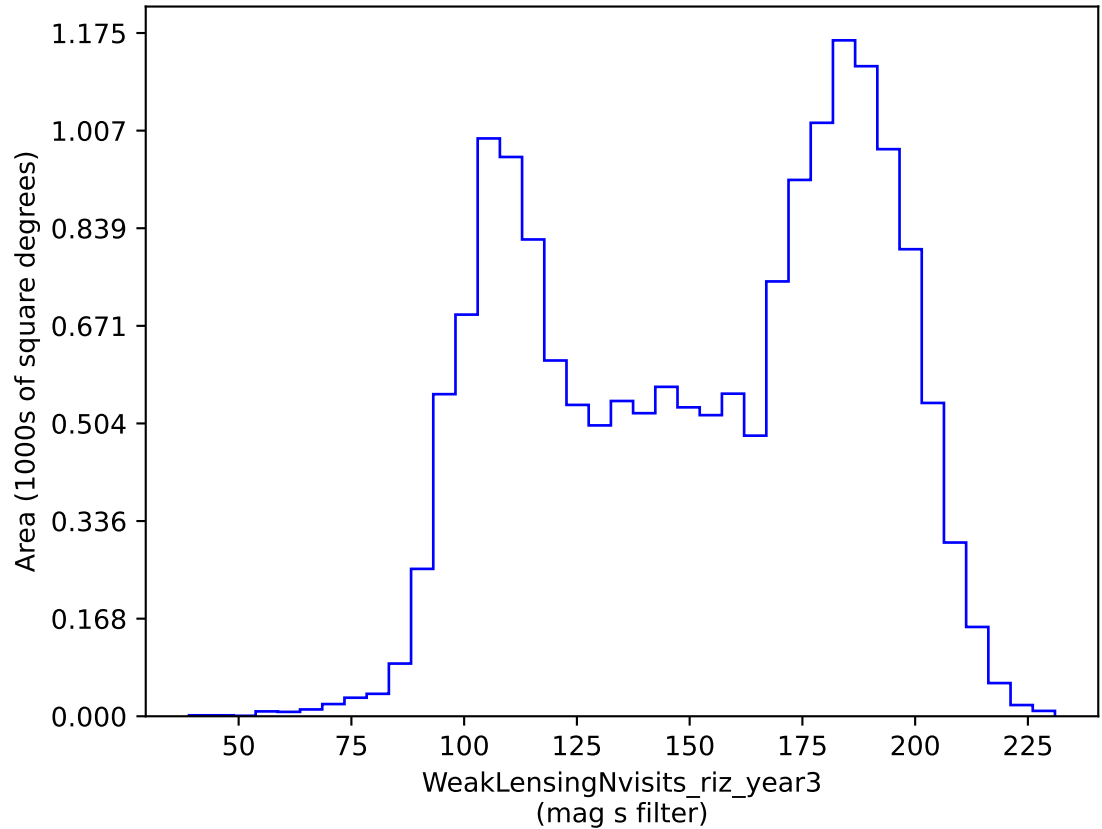
weather_cloudso8v3.4_10yrs gri band non-DD: WeakLensingNvisits_riz_year3
