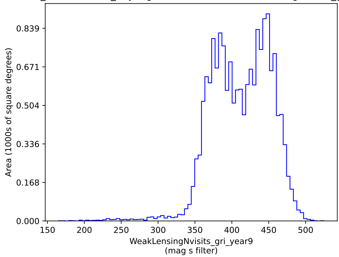
weather_cloudso8v3.4_10yrs gri band non-DD: WeakLensingNvisits_gri_year9
