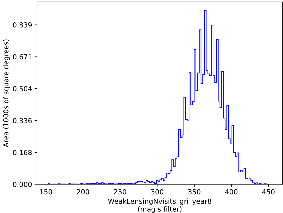
weather_cloudso8v3.4_10yrs gri band non-DD: WeakLensingNvisits_gri_year8
