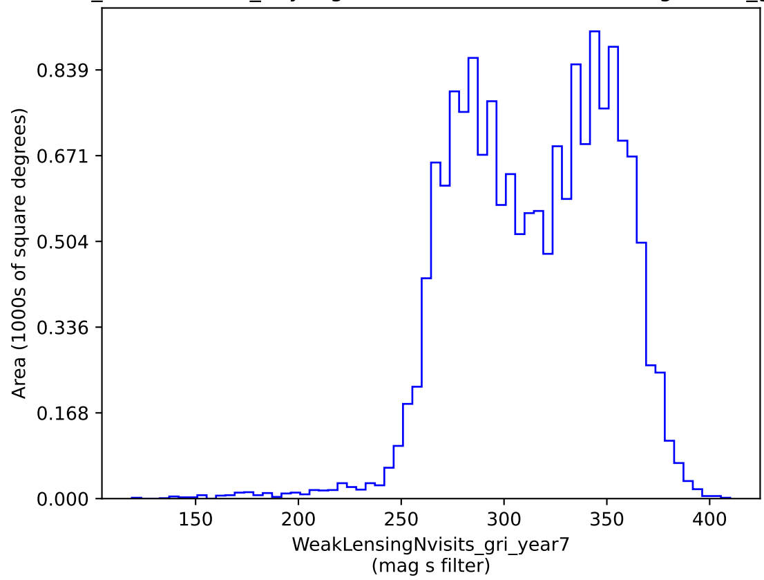
weather_cloudso8v3.4_10yrs gri band non-DD: WeakLensingNvisits_gri_year7
