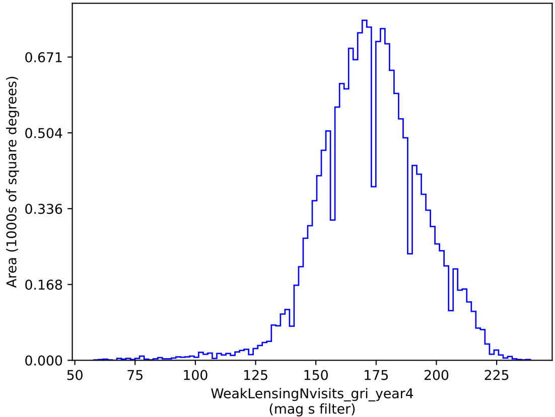
weather_cloudso8v3.4_10yrs gri band non-DD: WeakLensingNvisits_gri_year4
