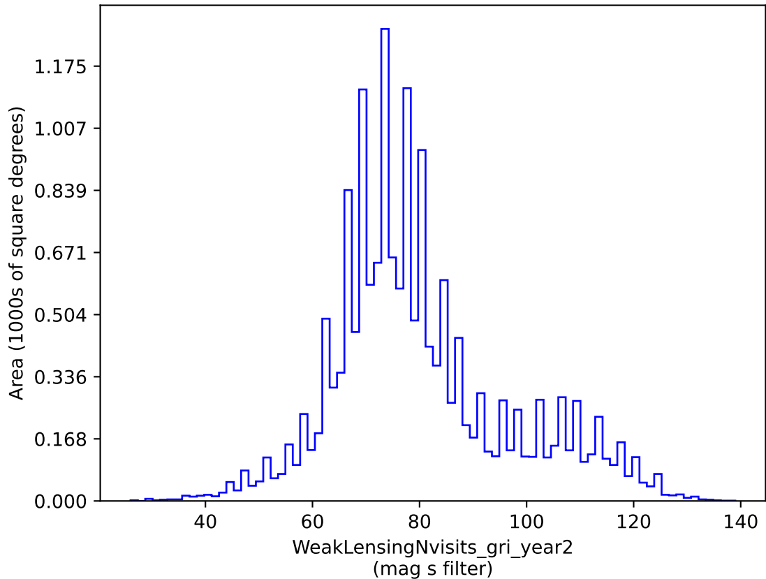
weather_cloudso8v3.4_10yrs gri band non-DD: WeakLensingNvisits_gri_year2
