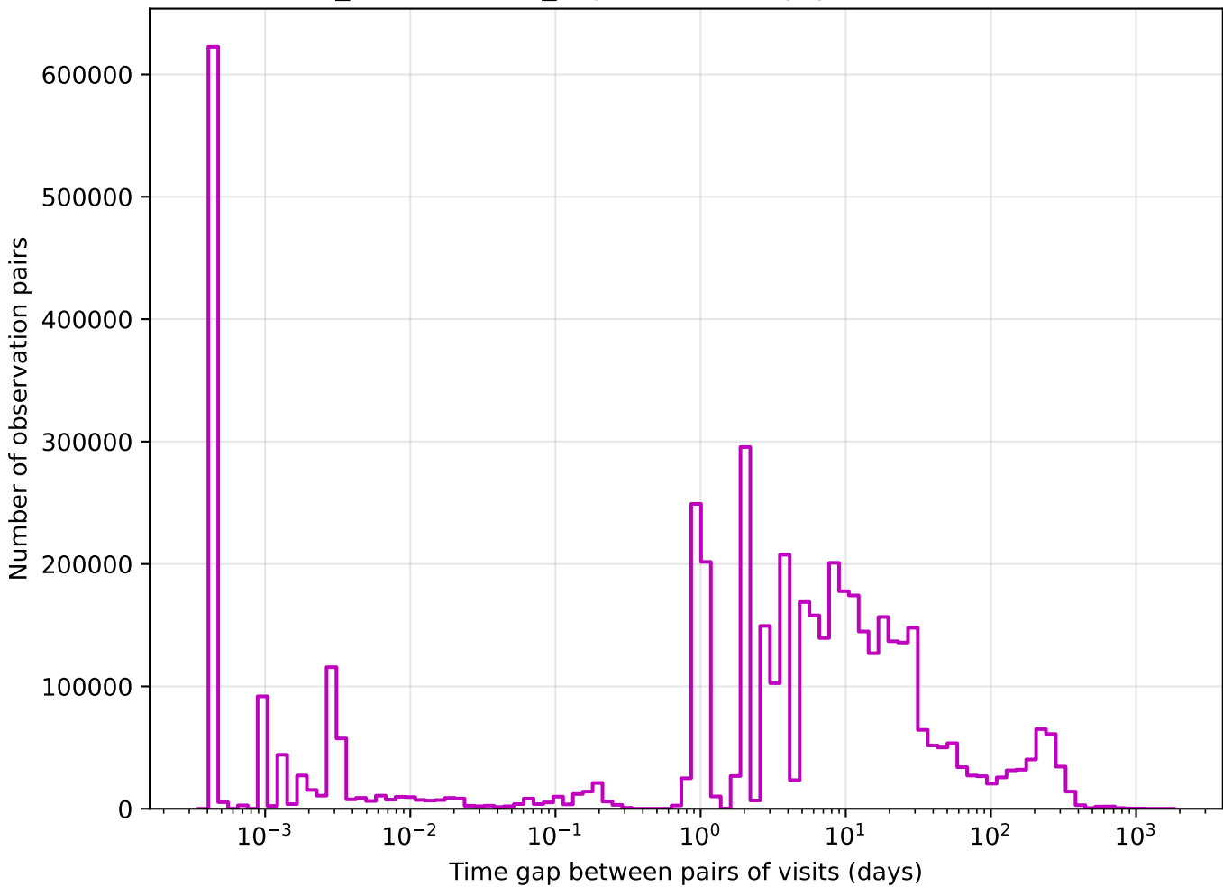
weather_cloudso8v3.4_10yrs z band: Tgaps observationStartMJD
