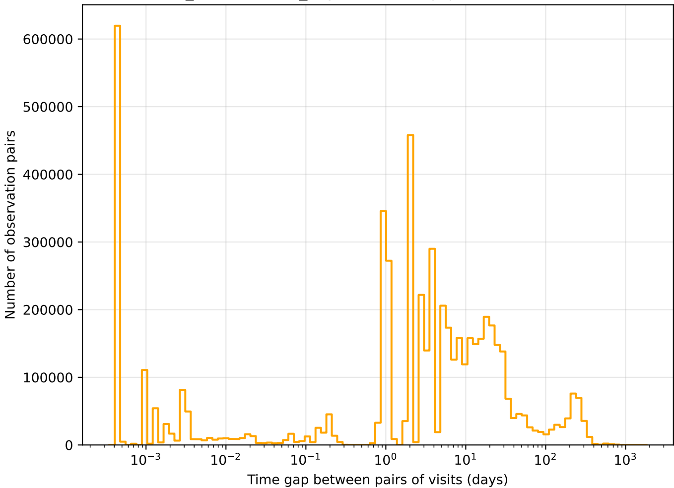
weather_cloudso8v3.4_10yrs r band: Tgaps observationStartMJD
