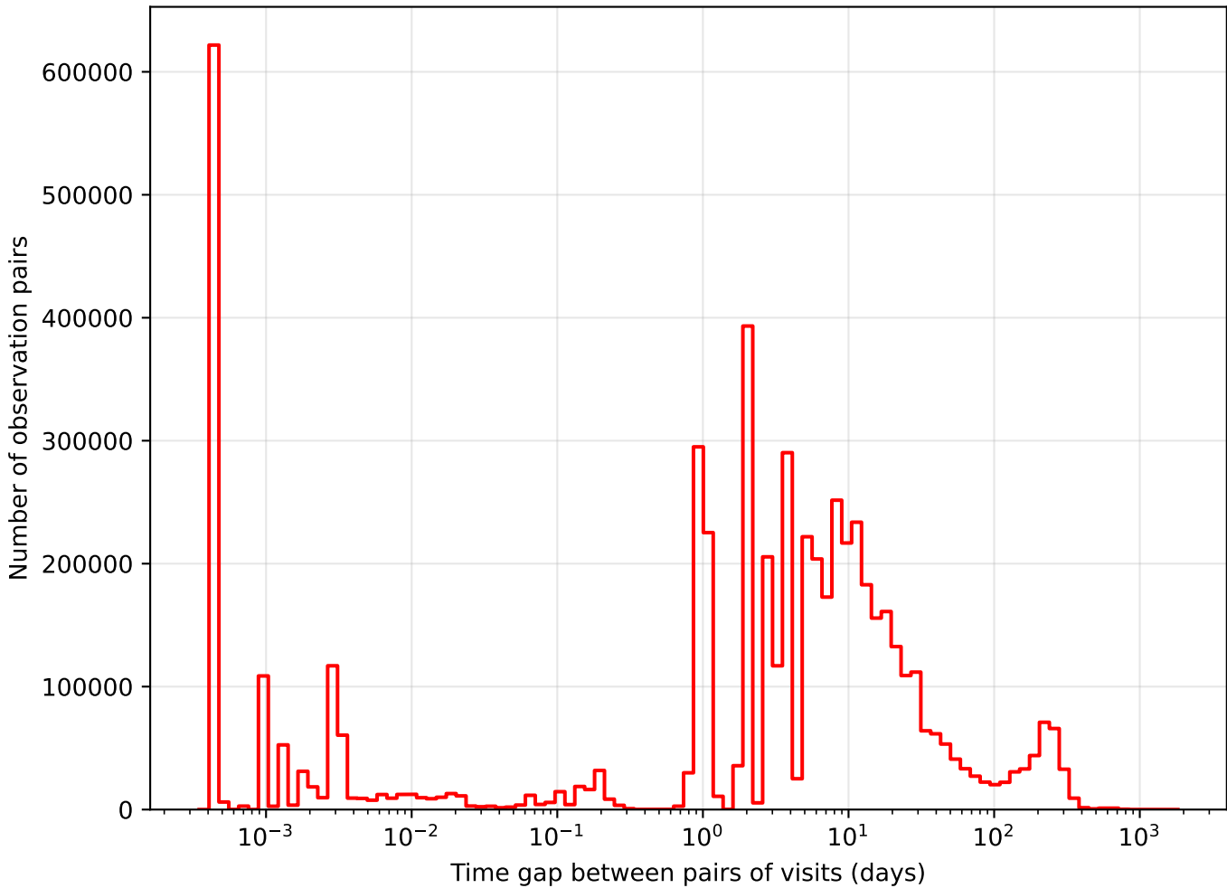
weather_cloudso8v3.4_10yrs i band: Tgaps observationStartMJD
