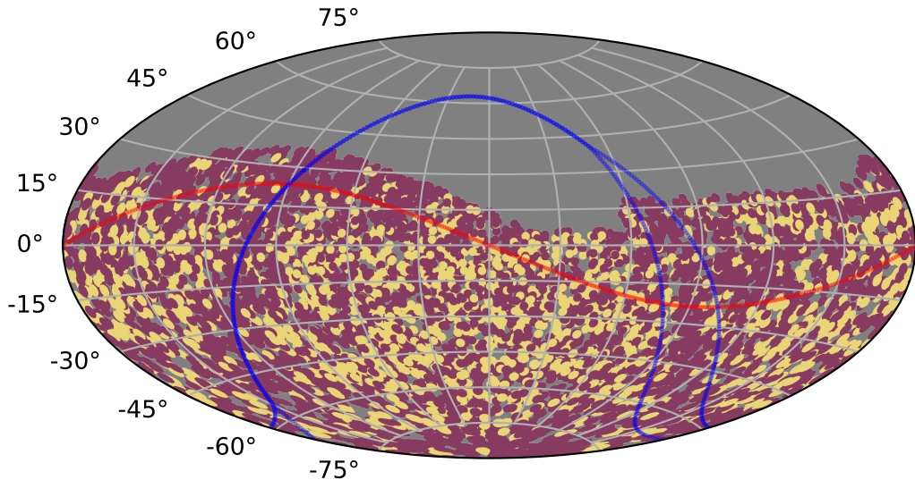
weather_cloudso8v3.4_10yrs : TDEsPopMetric_prepeak
