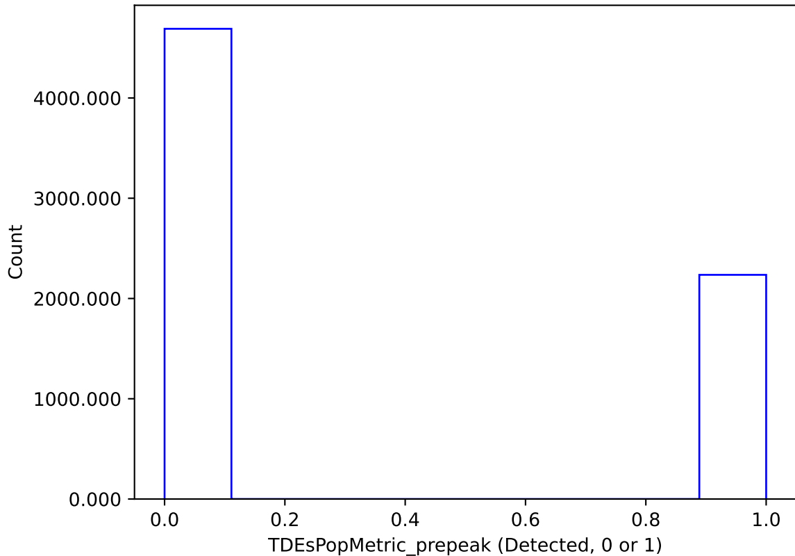
weather_cloudso8v3.4_10yrs : TDEsPopMetric_prepeak
