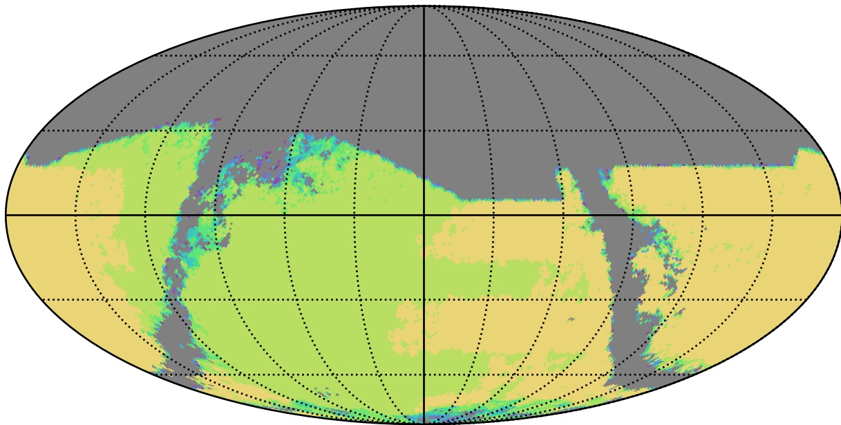
weather_cloudso8v3.4_10yrs : TDC_campaign
