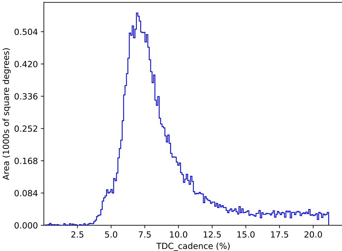
weather_cloudso8v3.4_10yrs : TDC_cadence
