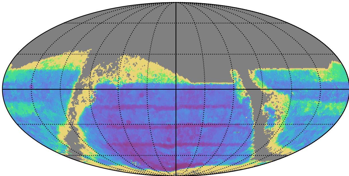
weather_cloudso8v3.4_10yrs : TDC_accuracy
